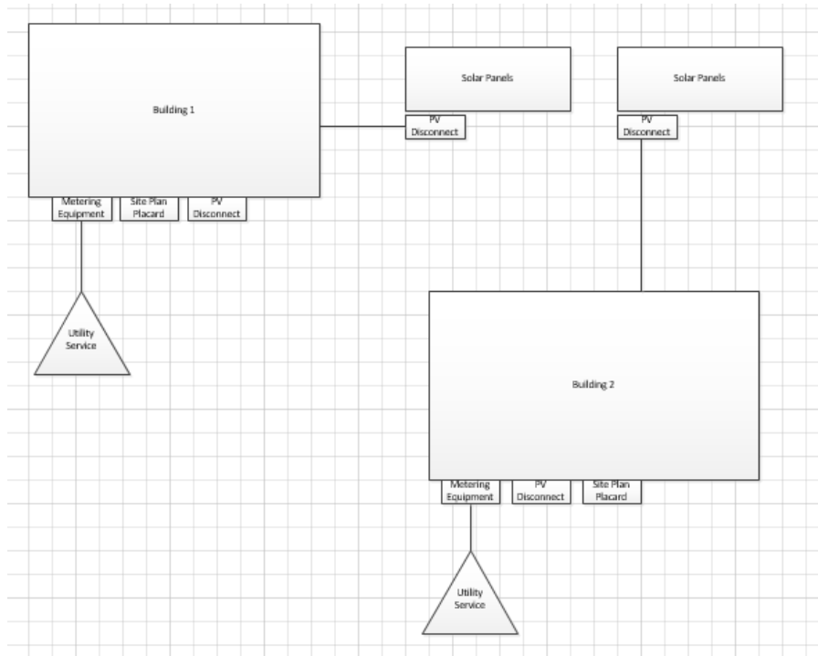
Figure 4: Two buildings on the same premise with multiple ground mounted customer-owned generation.
