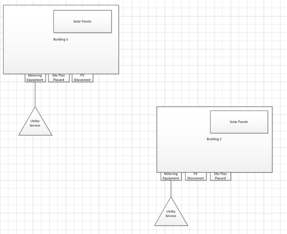
Figure 3: Two buildings with customer-owned generation on one premise.
