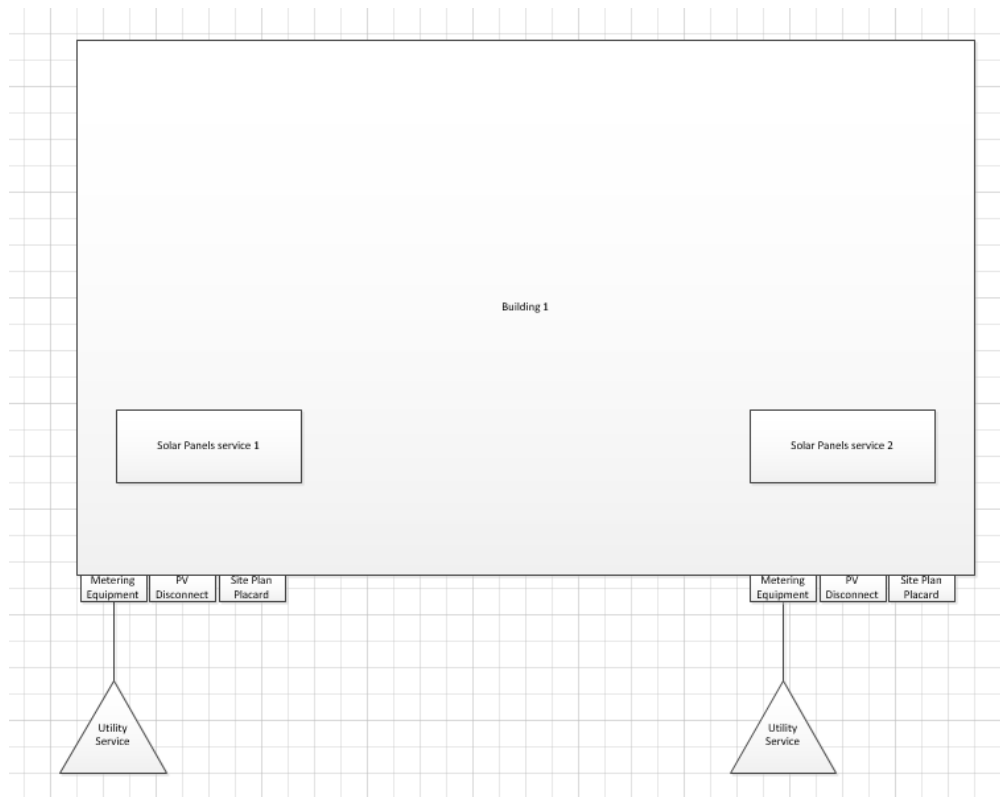
Figure 5: One large building with two services each with customer-owned generation interconnected.
