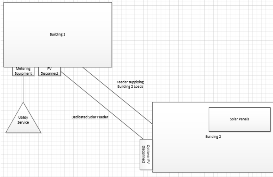
Figure 2: Building with customer-owned generation fed by another building with a dedicated solar feeder
